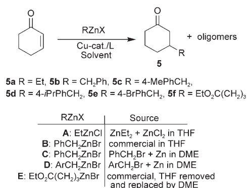
Scheme 3. Organozinc addition to 2-cyclohexenone (in D , Ar = 4-Me, 4- i Pr, 4-Br).
